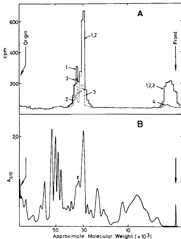
Fig.1. Distribution of radioactivity due to [ ^{14}\text{C} ]NSPM in 117 \mu\text{g} submitochondrial particles (A), and distribution of the particle protein (B). Submitochondrial particles were incubated as follows: 0.88 mg particles were added to 1 ml solution containing 0.25 M sucrose, 50 mM Tris-acetate, 30 mM \text{MgCl}_2 , 40 mM phosphate, 12.5 mM ATP (pH 7.5) at 0^\circ\text{C} . (1) (solid line) [ ^{14}\text{C} ]NSPM was added after 10 min incubation at 0^\circ\text{C} and 1 min at 37^\circ\text{C} to 20 nmol/mg protein and the reaction stopped after 2 min at 37^\circ\text{C} with 1 mM cysteine. (2) (dotted line) as (1) but 10 min preincubation of the particles at 0^\circ\text{C} and 1 min at 37^\circ\text{C} with 230 nmol diamide/mg protein. (3) (dashed line) as (2) but preincubation with 26 nmol CAT/mg protein. The protein distribution pattern of submitochondrial particles is unchanged by the incubation procedures, the scan shown in fig.1B corresponds to fig.1A, trace 3.
